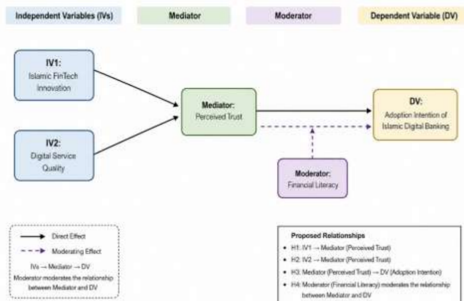
Figure 01: conceptual model
