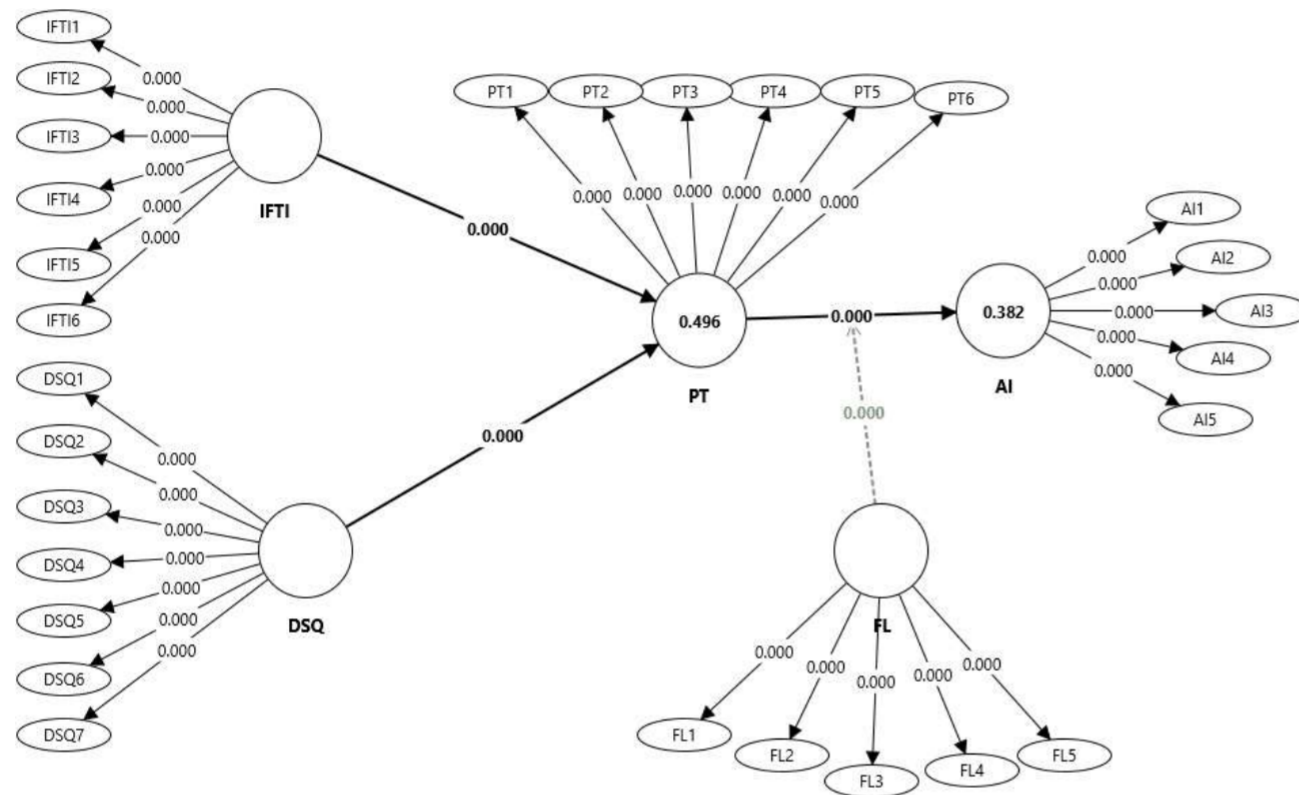
Figure 03: Structural Model
